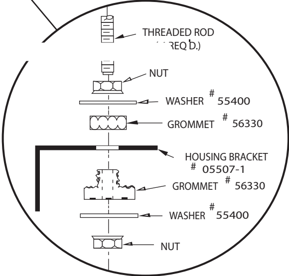
" Vibration Isolator Mount Detail " ( 4 REQUIRED )
