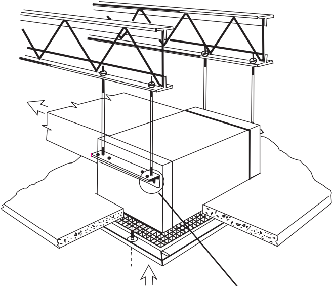
VIBRATION HANGER CEILING MOUNTING
