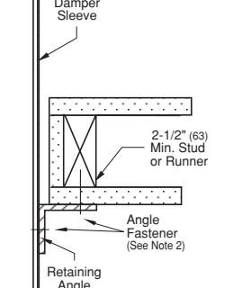
Single-Side System
